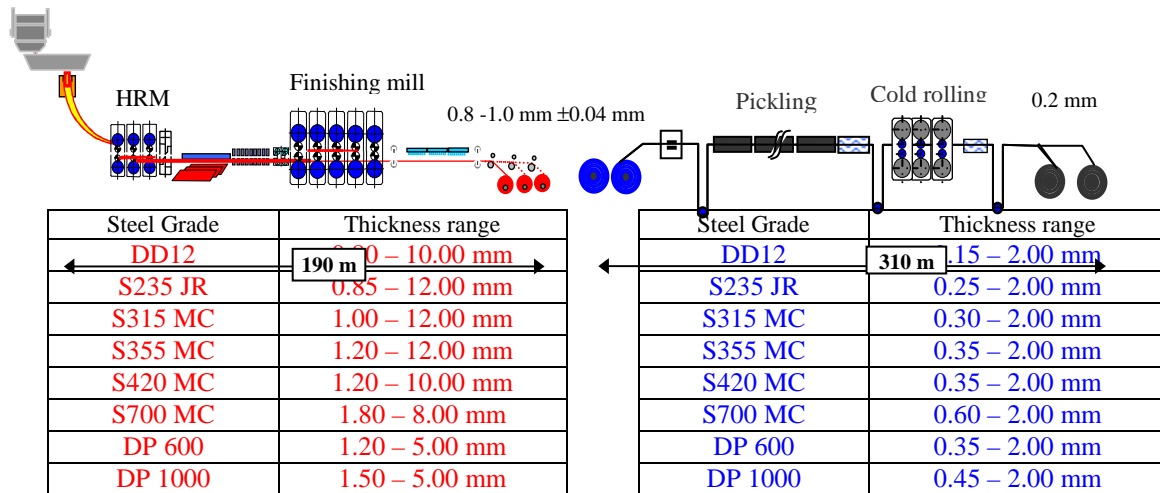
Figure 8: Hot and Cold Rolled products
