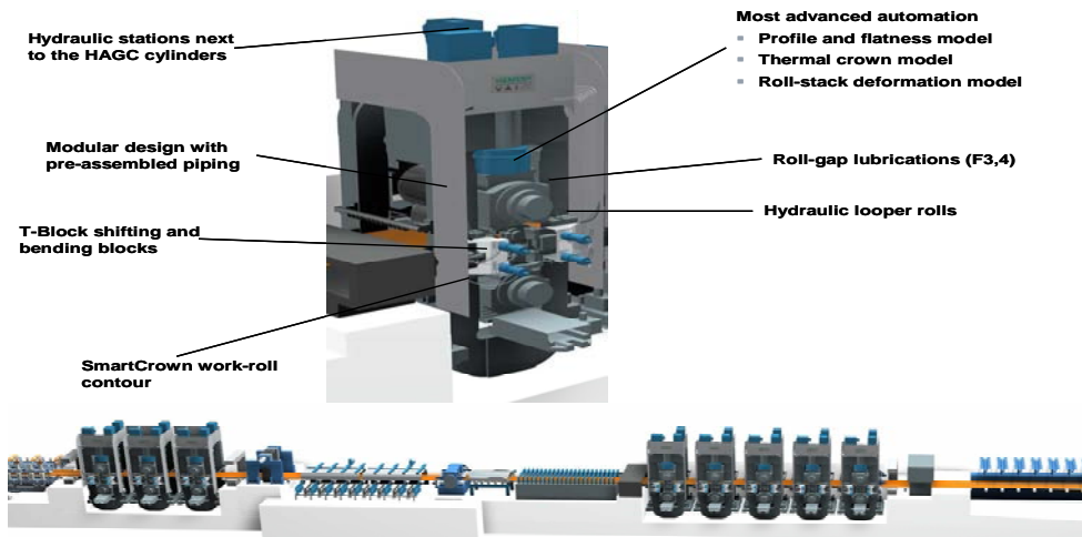
Figure 5: Application of SmartCrown® Technology
