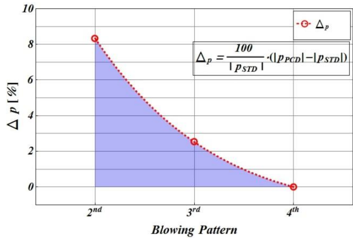
Figure 5. Pressure Difference for Different Blowing Patterns.
