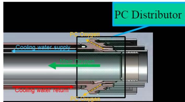
Figure 2. Diversion of Oxygen for Post – Combustion from the Main Oxygen Flow. Source: Tallman Bronze
