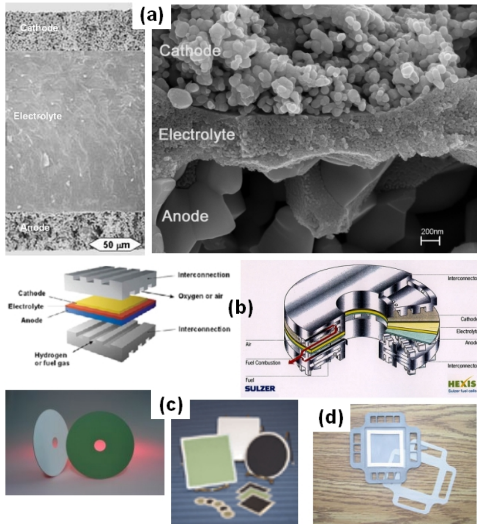
Figure 5. SOFC features: (a) scanning electron microscopy images show the EEA structures; (b) fuel cell assembly schemes; (c) EEA components, (d) ceramic interconnector.
