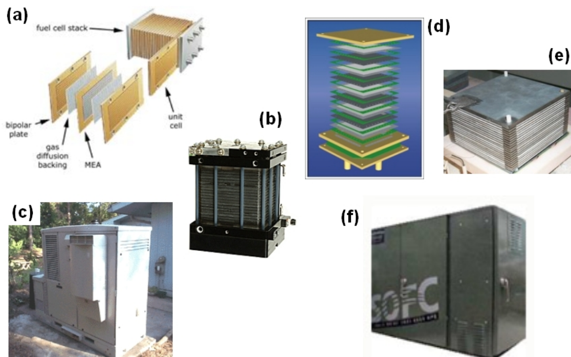
Figure 1. PEMFC (a, b, c) and SOFC (d, e, f) systems: (a) and (d) stack schemes; (b) and (e) stack examples; (c) and (f) generation units.
