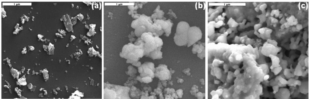
Figure 6. SOFC powders: (a) YSZ synthesized by GNP; (b) YSZ synthesized by Sol-Gel method; (c) lanthanum manganite cathode synthesized by combustion method.
