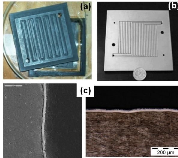
Figure 3. PEMFC bipolar plates: (a) graphite-based bipolar plate; (b) metallic bipolar plate, (c) scanning electron and optical microscopy images show different coatings on stainless steel bipolar plates.
