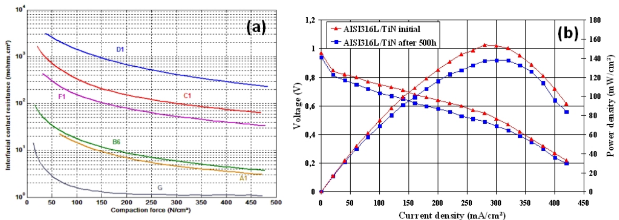
Figure 4. (a) ICR values against compression force. Samples: A1 (titanium nitride), B6 (chromium nitride), C1 (ion nitrided), D1 (diamond-like carbon), F1 (without coating) and G (conventional graphite for PEMFC bipolar plates); (b) PEMFC with AISI316L/TiN plates - Initial and after 500 hours of operation. (17)
