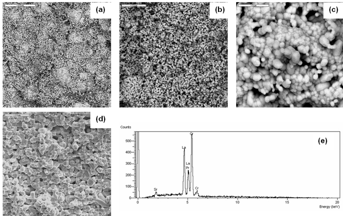
Figure 8. Microstructural characterization (SEM) of lanthanum chromite-based ceramics in different sintering conditions: (a) \text{La}_{0.90}\text{Ca}_{0.10}\text{CrO}_3 -1.200 C, (b) \text{La}_{0.90}\text{Sr}_{0.10}\text{CrO}_3 - 1.300 C, (c) \text{La}_{0.90}\text{Sr}_{0.10}\text{Cr}_{0.95}\text{Mg}_{0.05}\text{O}_3 – 300 C, (d) \text{La}_{0.90}\text{Ca}_{0.05}\text{Sr}_{0.05}\text{Cr}_{0.95}\text{Mg}_{0.05}\text{O}_3 – 1.400 C, (e) EDS analysis result of the microstructure shown in Figure 8(d).
