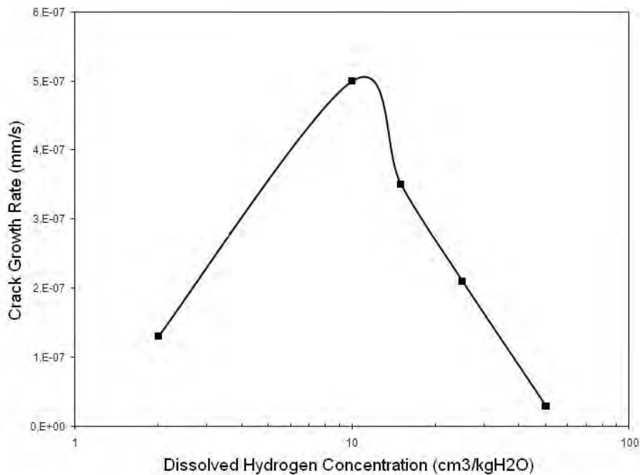
Figure 1. Experimental result for Alloy 182 SSR tested at 325°C in primary water with strain rate 3.10 -7 s -1 . (3)
