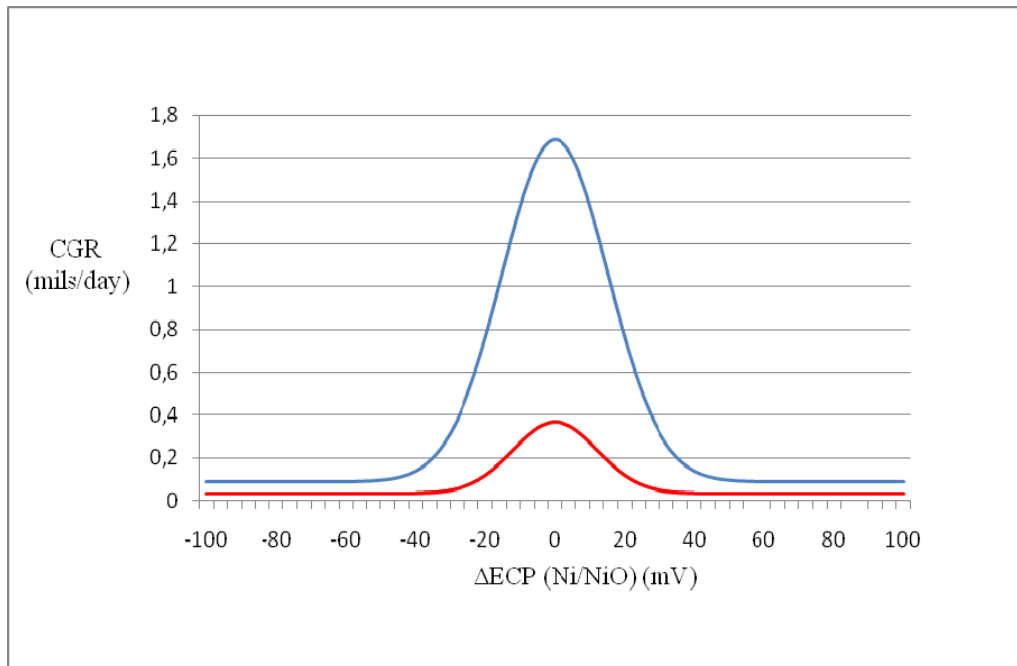
Figure 3. Equation 6 modeling fit to Alloy 182 CDTN data (blue) (3) compared to raw data from Andresen (red). (2) Plotted through Microsoft Excel 2007.
