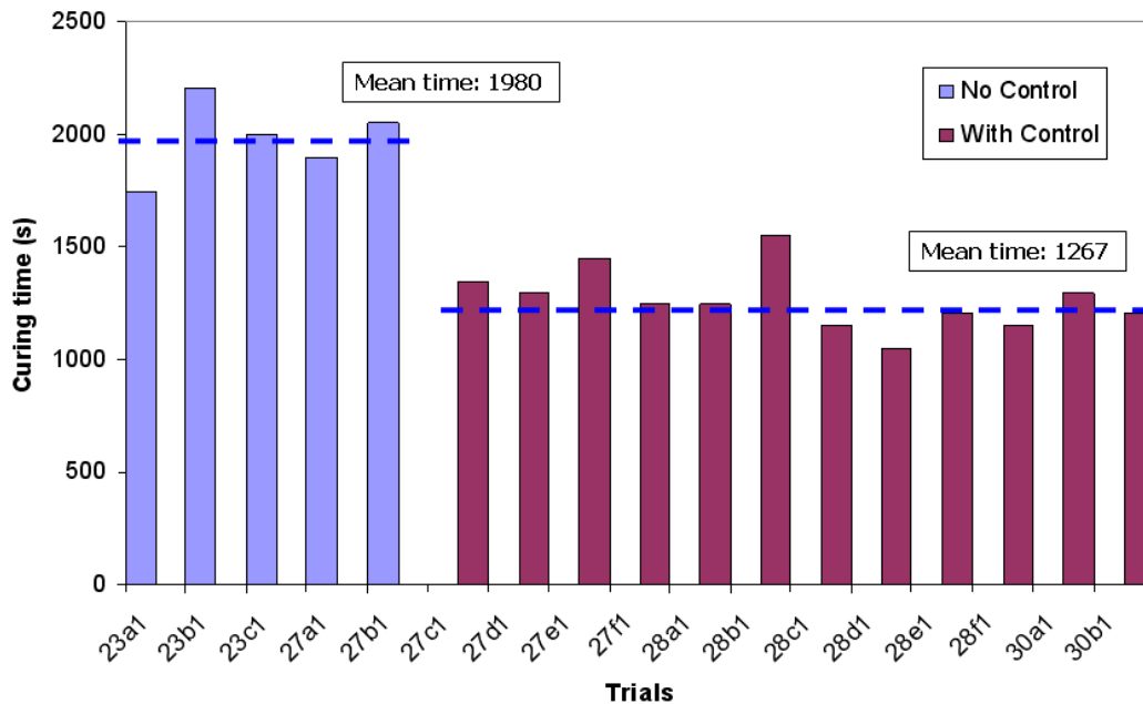
Fig.7. Curing times for an RTM production line before and after cure monitoring and control shows mean cure cycle time acceleration of 36%.
