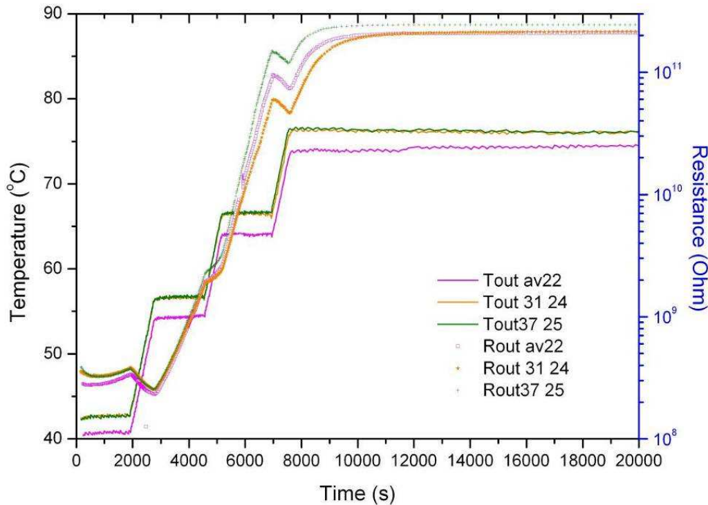
Fig.3. Electrical resistance and temperature during the curing of an epoxy system with nominal mixing ratio (av22), 2.2% more hardener (Rout37 25) and 2.2% less hardener (Rout31 24).
