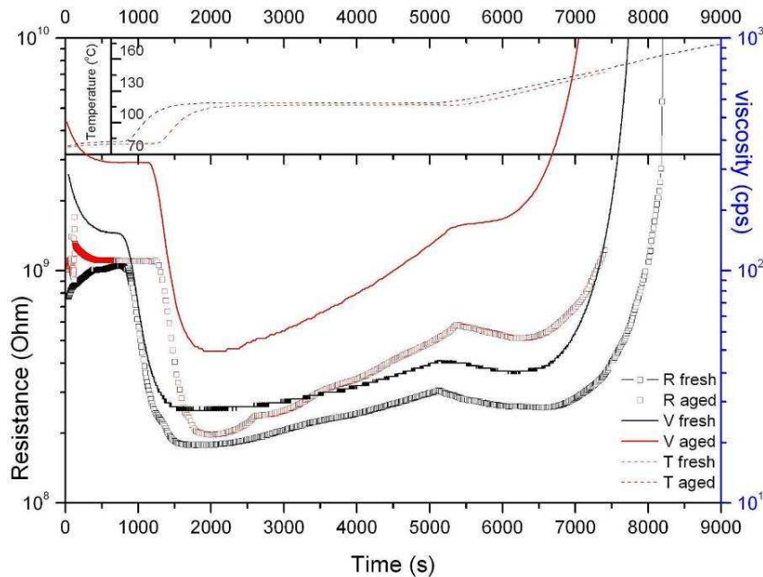
Fig.4. Electrical resistance (symbols), viscosity (solid lines) and temperature (dashed lines) during the injection of a fresh and an expired monocomponent epoxy system.
