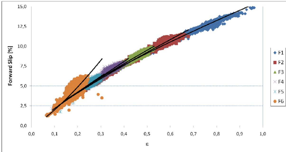
Figure 6: Forward slip in function of strain degree \epsilon for the six rolling stands of the finishing mill.
