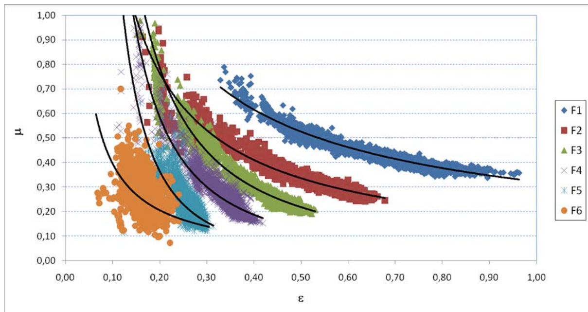
Figure 2: Friction coefficient \mu in function of strain degree \epsilon for the six rolling stands of the finishing mill.
