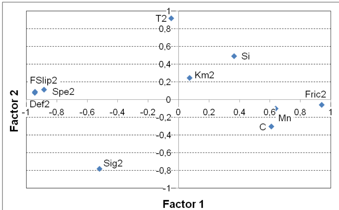
Figure 1: Results of the principal components analysis determined from F2 stand rolling data. Legend: C , carbon content; Mn , manganese content; Si , silicon content; T2 , rolling temperature; Def2 , strain degree, Km2 , length of strip processed up to that moment by the work rolls; FSlip2 , forward slip; Sig2 , hot strength; and Fric2 , friction coefficient.
