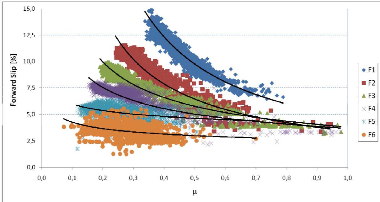
Figure 4: Forward slip in function of friction coefficient \mu for the six rolling stands of the finishing mill.
