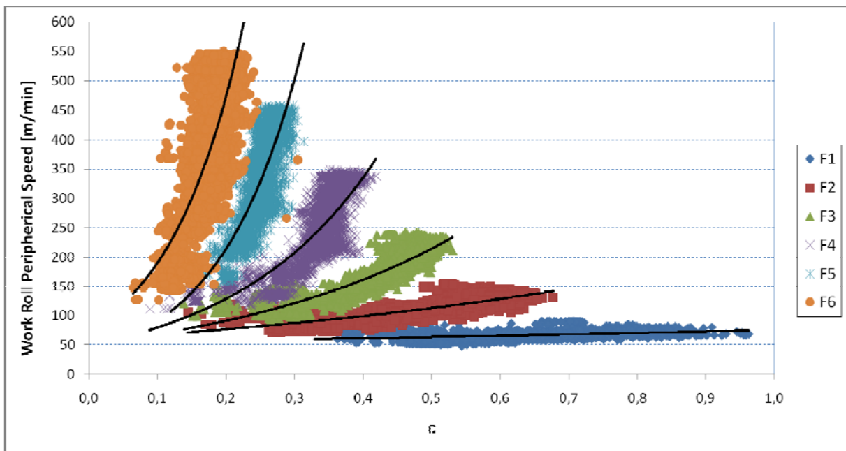
Figure 5: Work roll peripheral speed in function of strain degree \epsilon for the six rolling stands of the finishing mill.
