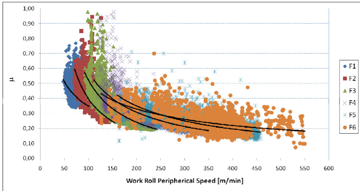
Figure 3: Friction coefficient \mu in function of work roll peripheral speed for the six rolling stands of the finishing mill.
