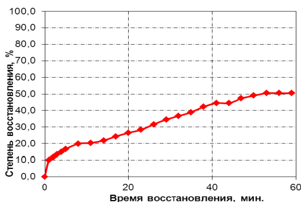
Figure 4. Reducibility curve for brex #3.02.
