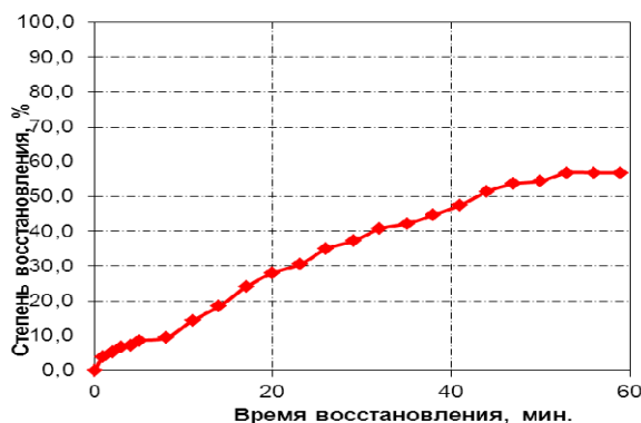
Figure 5 Reducibility curve for brex #3.06.
