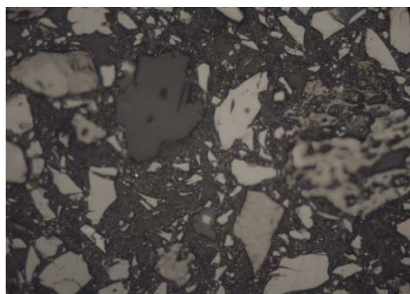
Figure. 3 Microstructure of the initial brex #4, magnification 500 (Light – particles of the magnetite concentrate, Light-gray – coke particles, dark-gray cement binder).
