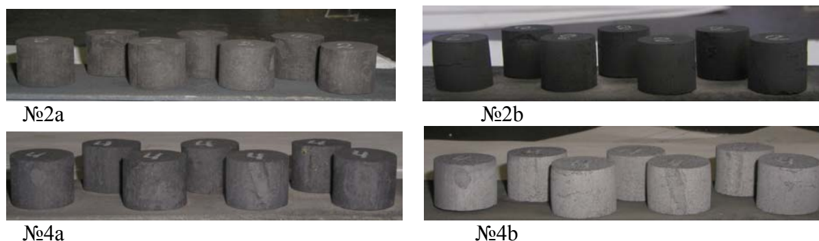
Figure 2. Samples of the brex #2 and #4 before (a) and after (b) thermal treatment under reducing atmosphere.
