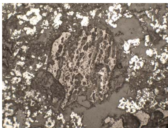
Figure. 4 Microstructure of the brex #4 after reduction, magnification 200. (gray – particles of the metallized iron, gray fields-- iron-silicate matrix, light-gray particles - coke).
