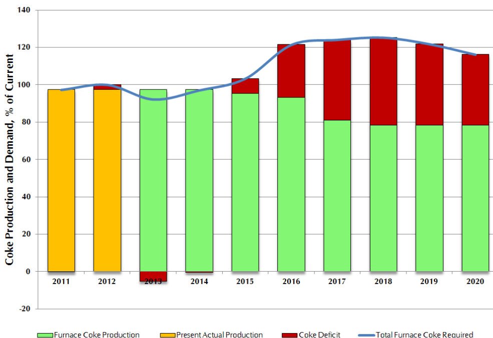
Figure 5 Furnace Coke Production versus Consumption
