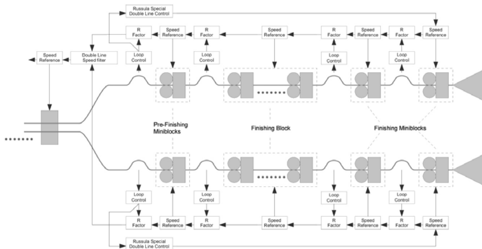
Figure 7. Two strand wire mill control diagram
