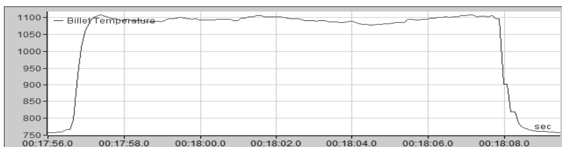
Figure 5. Uniform billet temperature graph.
