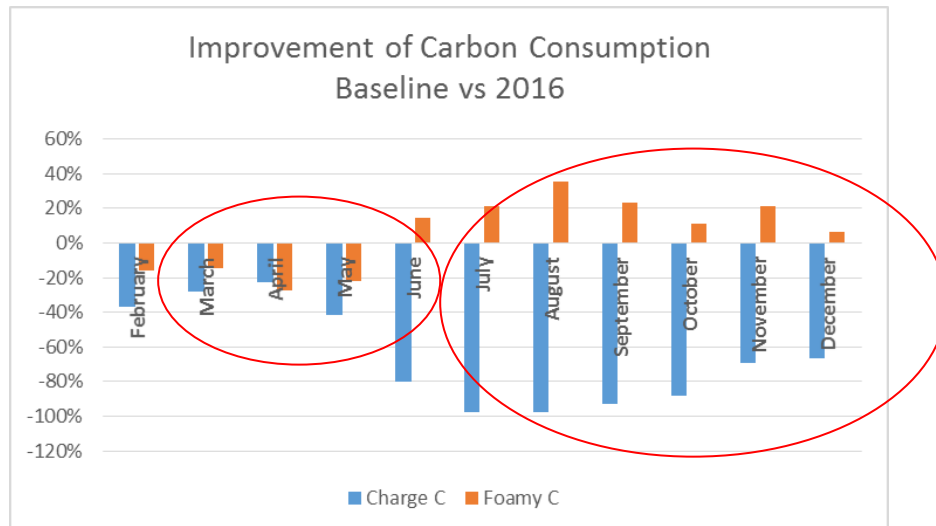
Figure 5. Carbon Consumption at Gerdau Monroe vs. Established Baseline.
