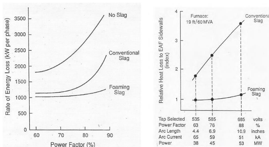
Figure 9. Established Benefits of Foamy Slag on Electrical Energy Consumption in EAF Steelmaking v
