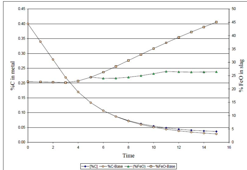
Figure 7. Simulation of EAF refining period iv
