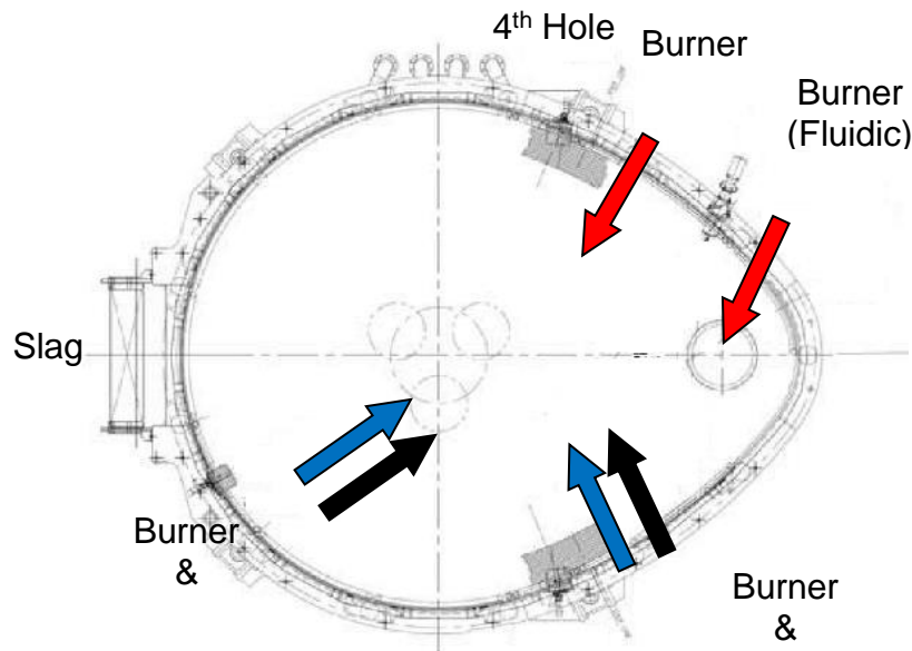
Figure 4. Top view of EAF at Gerdauro Monroe.
