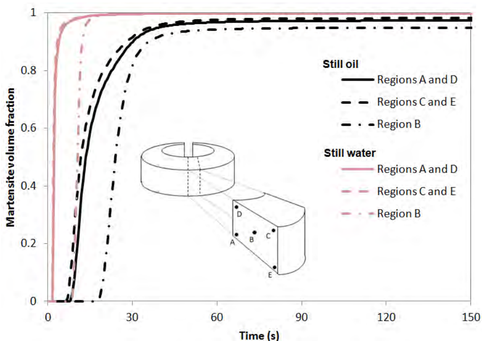
Figure 10. Simulated evolution of the martensite volume fraction at several points in the transversal cross-section of the C-ring during oil quenching.
