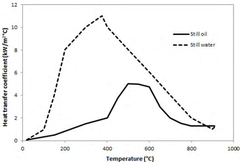
Figure 6. Heat transfer coefficient between AISI 4140 and two different quenchants: still oil and water. (11)
