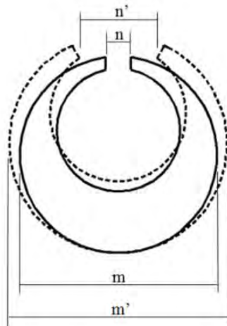
Figure 2. C-ring specimen before heat treatment ( m and n dimensions) and after heat treatment ( m' and n' dimensions).
