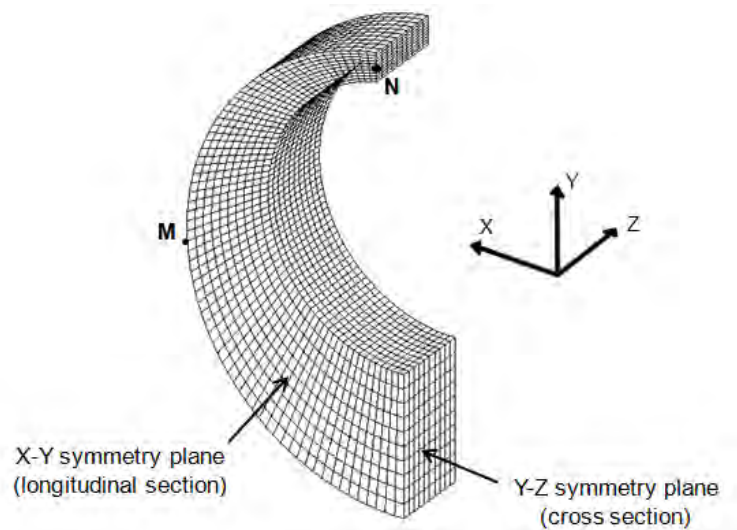
Figure 7. Meshed ¼ symmetric geometry, used for the simulation. Nodes M and N were used for outside diameter and gap opening evaluation, respectively.
