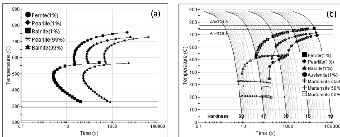
Figure 4. TTT and CCT diagrams of steel 4140 calculated by JMatPro.
