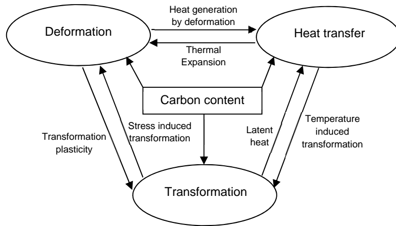
Figure 3. Coupled phenomena considered during the quenching simulations.
