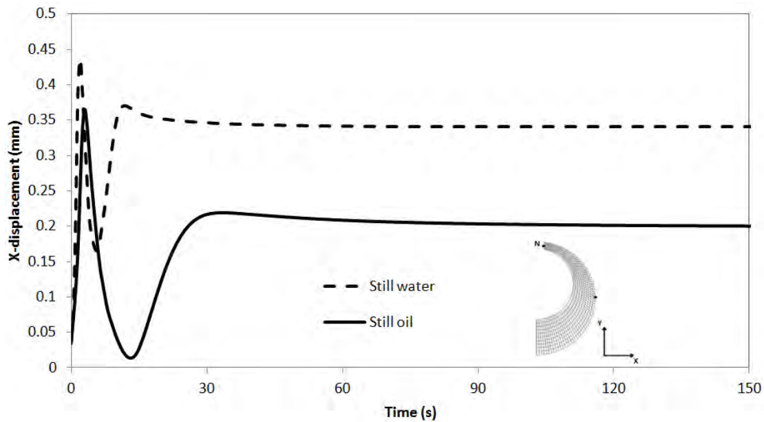
Figure 8. Simulated displacements in the x direction for Node N of the C-ring for still oil and water quenching processes.
