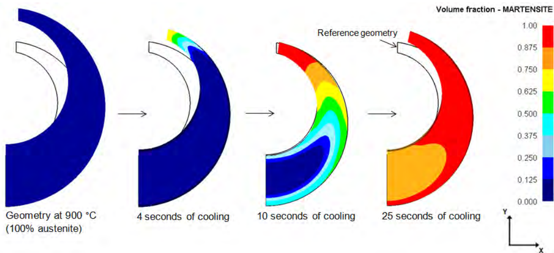
Figure 11. Martensite formation on the C-ring during the cooling simulation for oil quenching (displacement magnified 20x).
