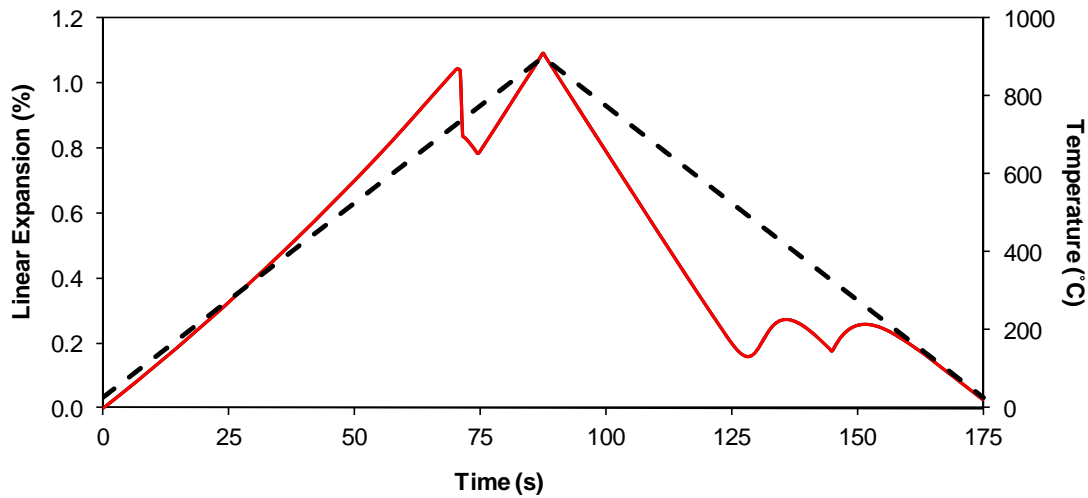
Figure 5. Linear expansion of alloy 4140 during a heating and cooling cycle, both at 10°C/s.
