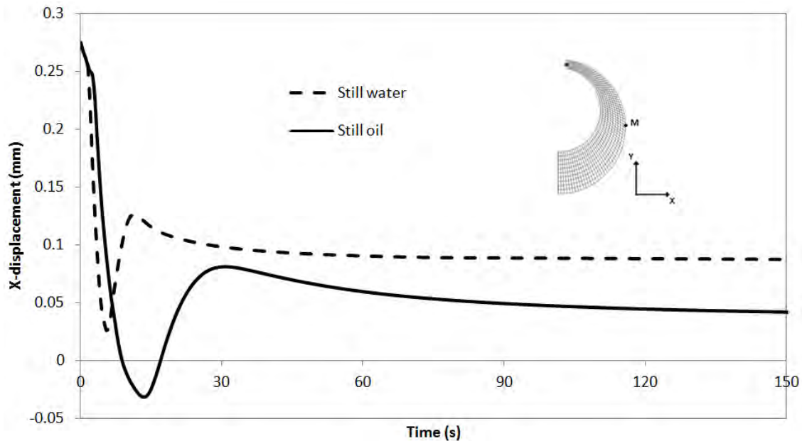
Figure 9. Simulated displacements in the x direction for Node M of the C-ring for still oil and water quenching processes.
