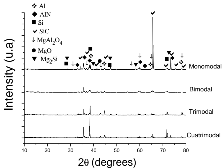
Figure 3 Typical diffractograms of composites with monomodal, bimodal, trimodal and cuatrimodal distributions.
