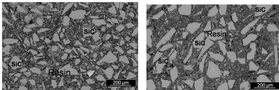
Figure 2. Representative photomicrographs of mounted specimens for pore size measurements.
