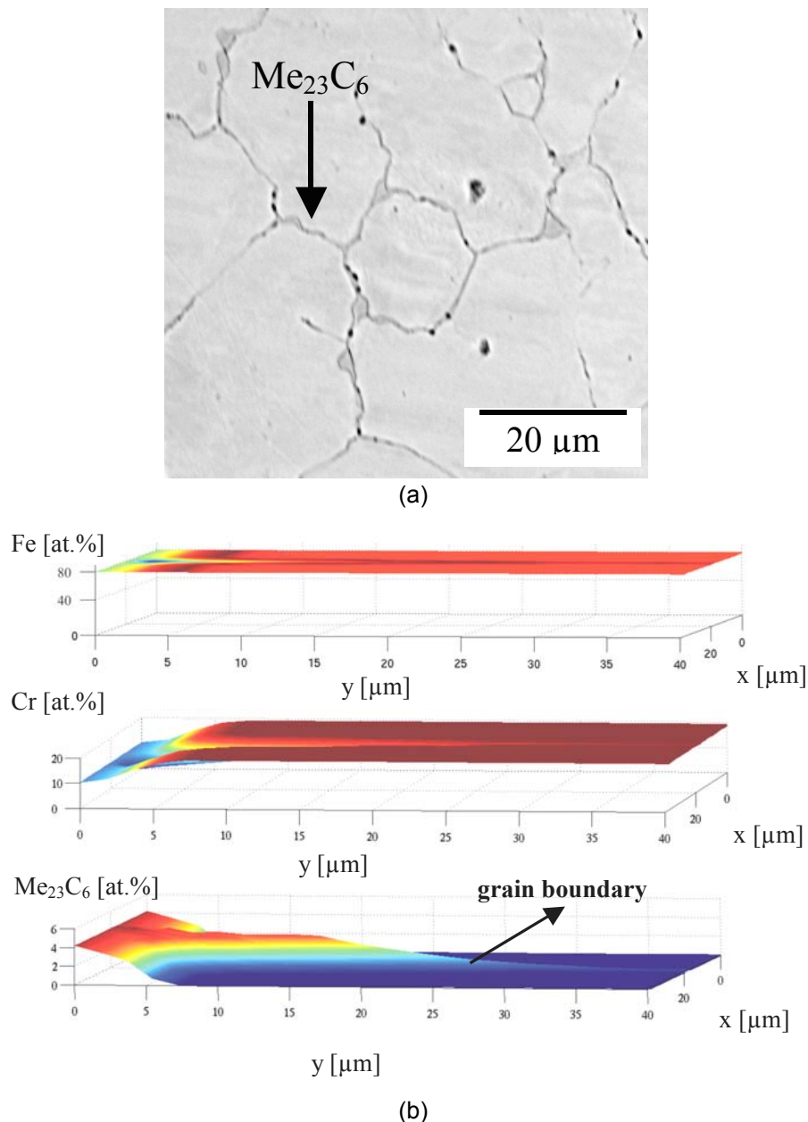
Figure 3. Initial stage of carbide formation in austenitic steel at 850°C during exposure to an He atmosphere containing 1vol% of methane for 10h: (a) cross section and (b) simulated concentration profiles.
