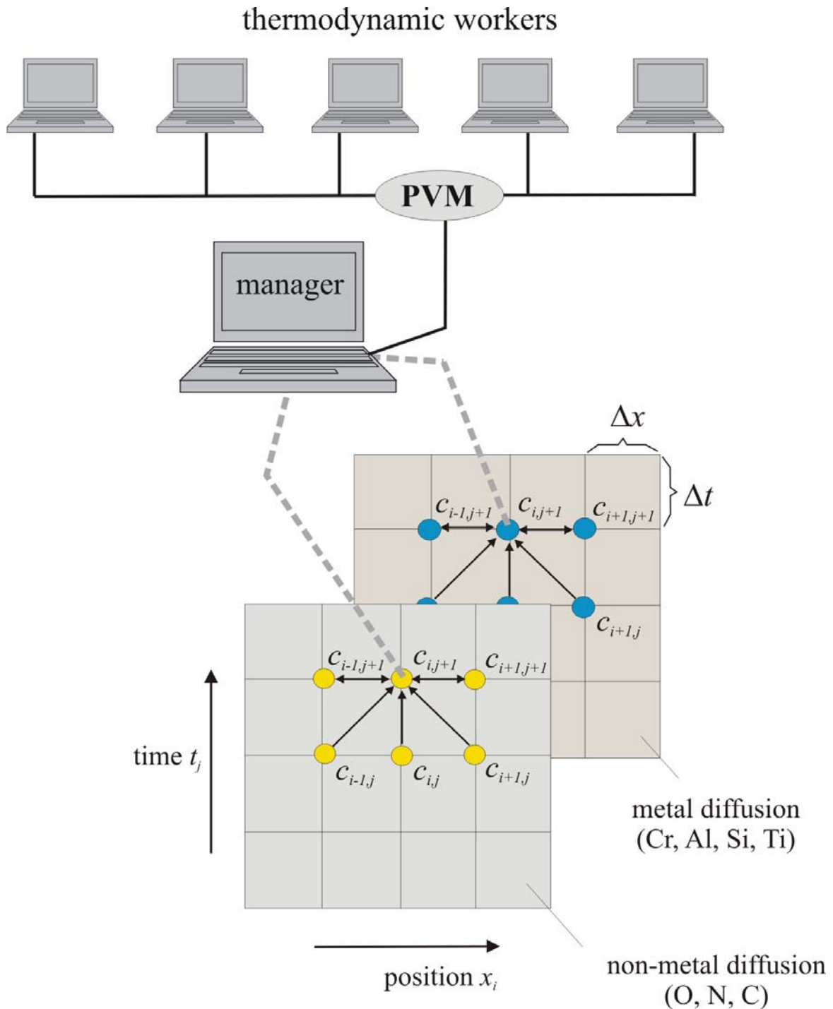
Figure 1. Schematic representation of the finite-difference technique (implicit Crank-Nicolson approach) in combination with the thermodynamic subroutine ChemApp.
