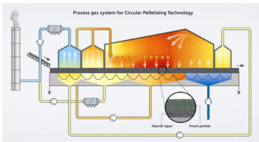
Figure 2. Schematic overview of the process gas flow in a CPT plant
