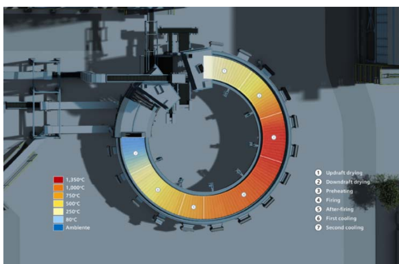
Figure 1: Process zones of the CPT induration furnace and respective temperature levels
