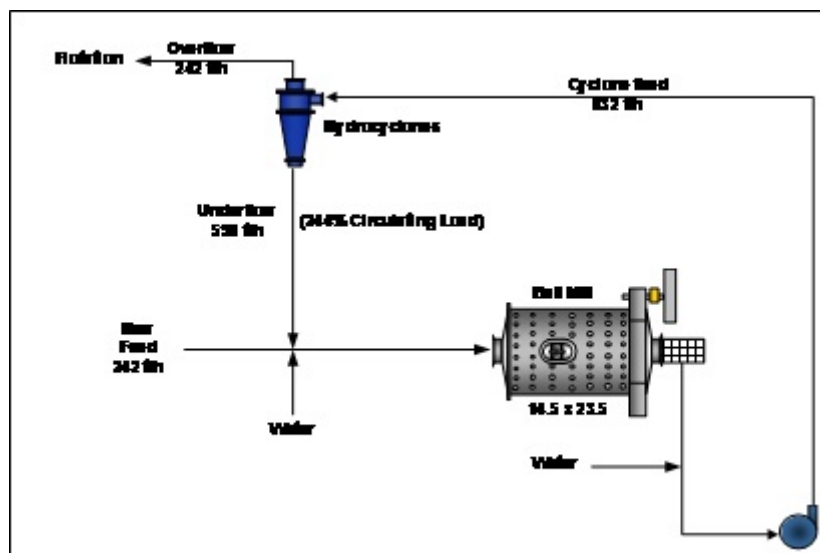
Figure 11. Cerro Lindo grinding circuit with hydrocyclone classification.
