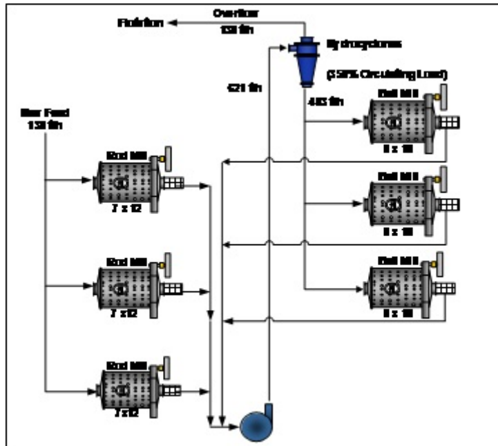
Figure 3. Brocal grinding circuit with hydrocyclone classification.
