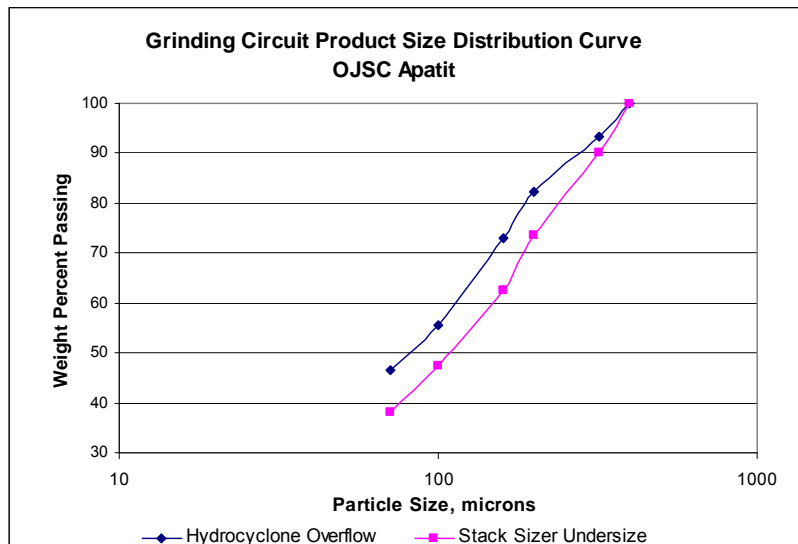
Figure 8. Comparison of circuit products from cyclone and screen circuits at OJSC Apatit.
