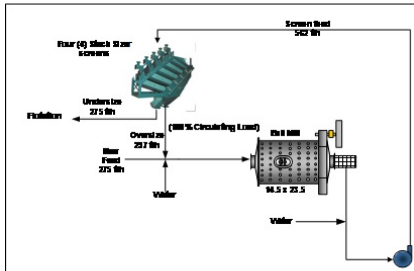
Figure 12. Cerro Lindo grinding circuit with screen classification.
