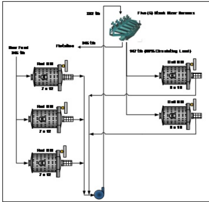
Figure 4. Brocal grinding circuit with screen classification.
